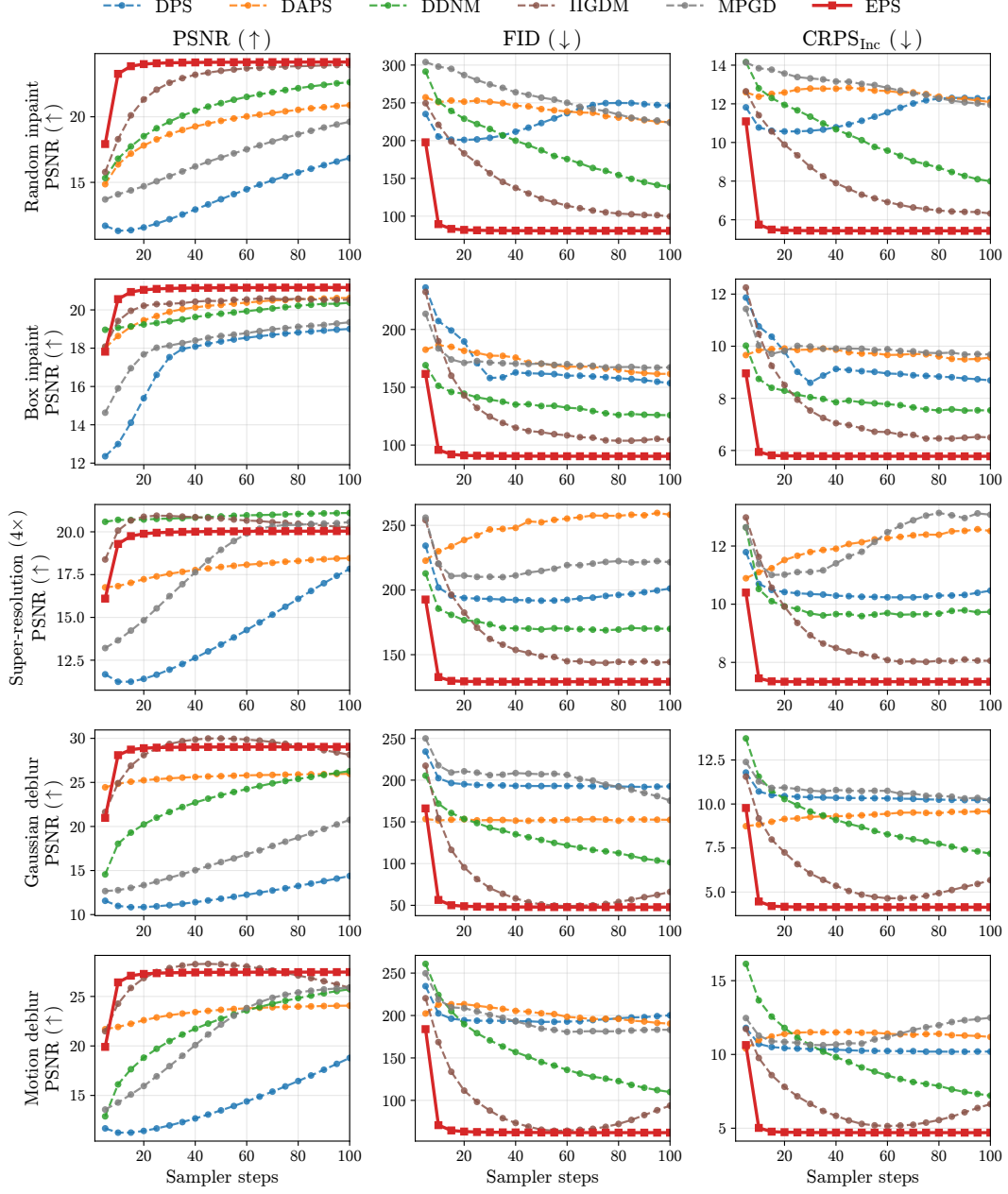
Figure 6: The plateau transfers to ImageNet-64. Sampling-step sensitivity on ImageNet-64; same layout as Fig. 5. EPS plateaus at the same step count on a more diverse class-conditional distribution, and the gap between EPS and the strongest sampling-based baseline (IIGDM) widens on the deblurring tasks.
