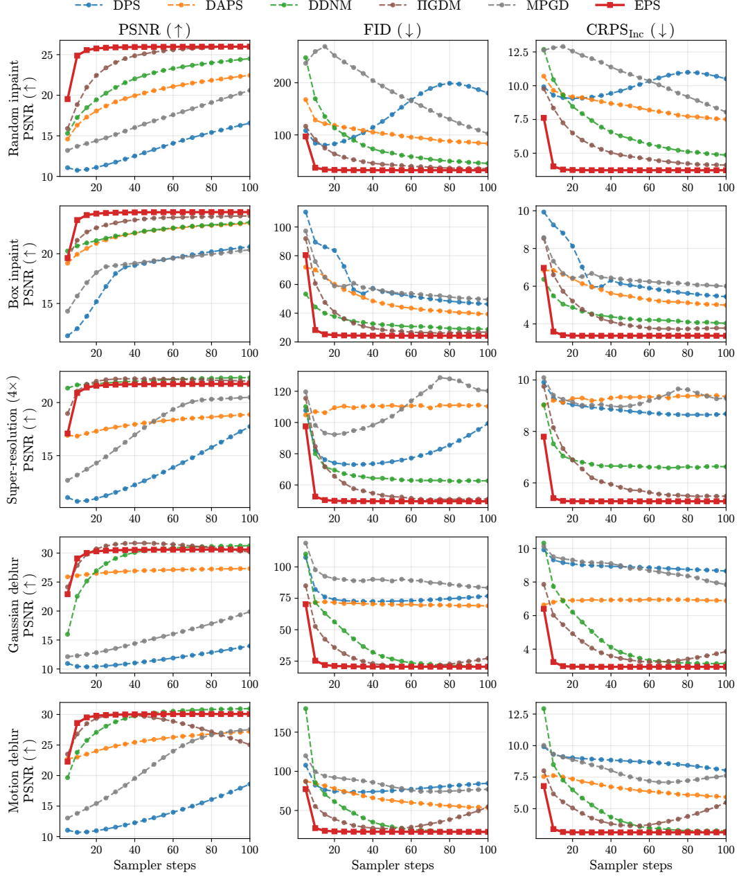
Figure 5: EPS plateaus by 15-20 steps on FFHQ-64. Sampling-step sensitivity on FFHQ-64 across the five tasks (rows). Columns report PSNR (↑), FID (↓), and Inception-feature CRPS (↓) versus sampler iterations under a 1-NFE-per-step Euler sampler. EPS reaches its asymptote within roughly 15-20 steps on every task and remains best or tied-best on FID and CRPS thereafter.
